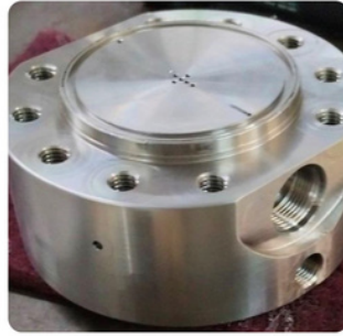
Liquid End Body-Hastelloy C
